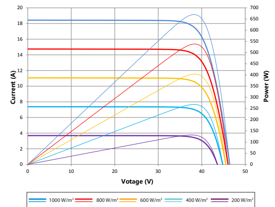
Current-Voltage & Power-Voltage Curve (670S)
